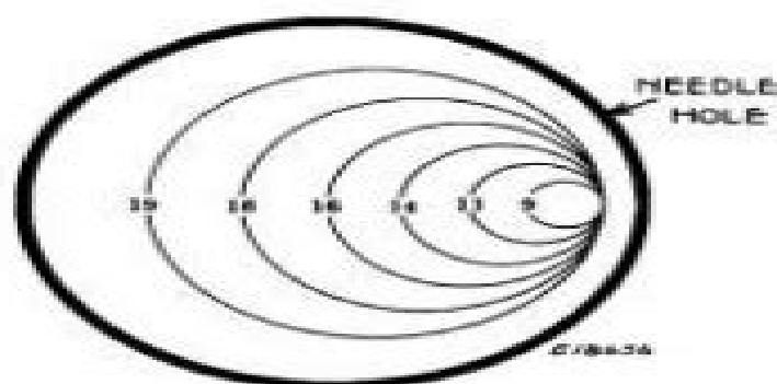
Fig. 15. Location of Needle in Relation to Throat Plate and Relative Positions of Each Size of Needle
