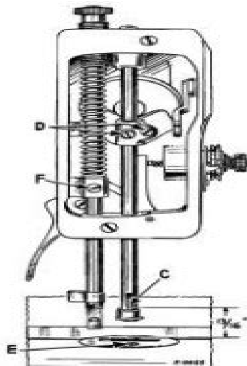
Fig. 14. Setting the Needle Bar
